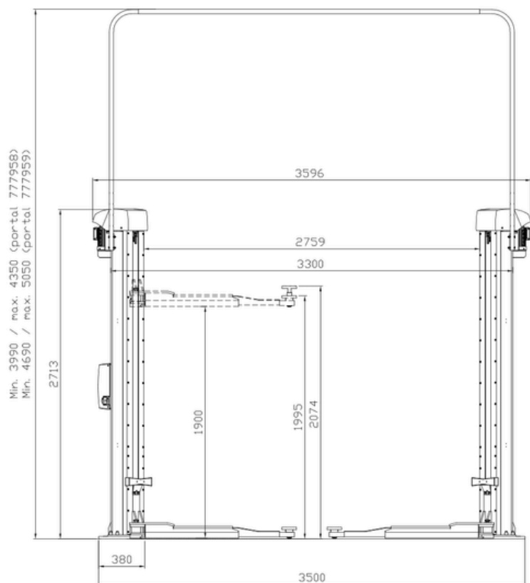
Short arm
