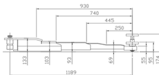
Short arm
